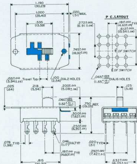
G-169 Four Pole/Three Position (with detent)
