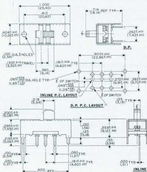
GPF-124 Single Pole Double Throw (with detent) GPF-126 Double Pole Double Throw (with detent)
