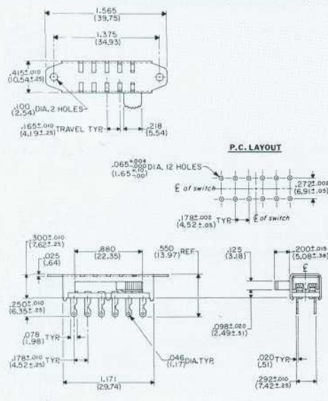
GI-163 Double Pole/Five Position (with detent)
