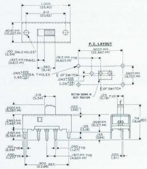
GP-132 Single Pole Double Throw (spring return)
