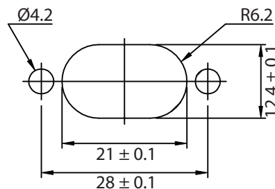
PANEL CUTOUT
