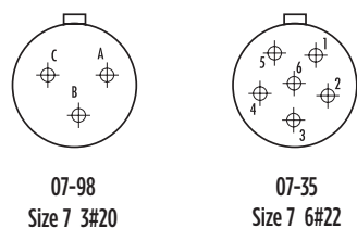
INSERT ARRANGEMENTS
