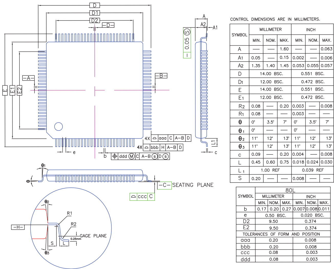
Figure 7-1. 80 LQFP package dimensions
