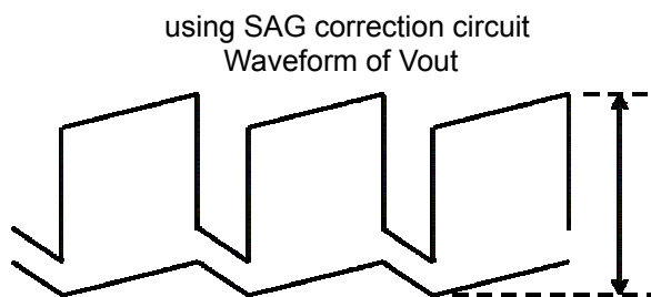
Waveform of Vout1
