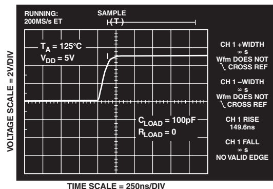
TPC 11. TMP04 Output Rise Time at 125°C
