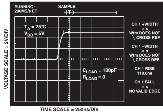
TPC 10. TMP04 Output Rise Time at 25°C
