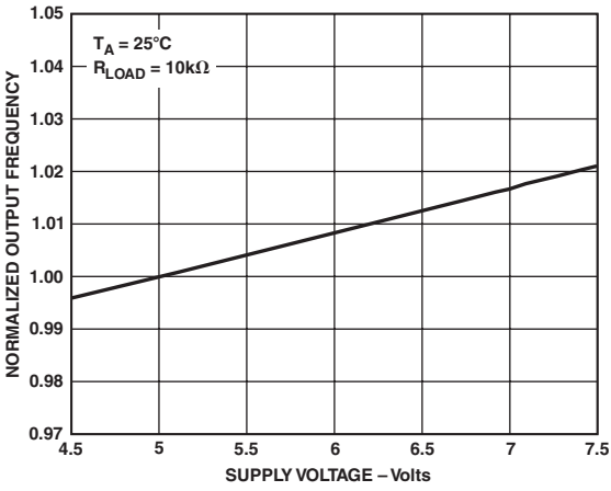
TPC 4. Normalized Output Frequency vs. Supply Voltage
