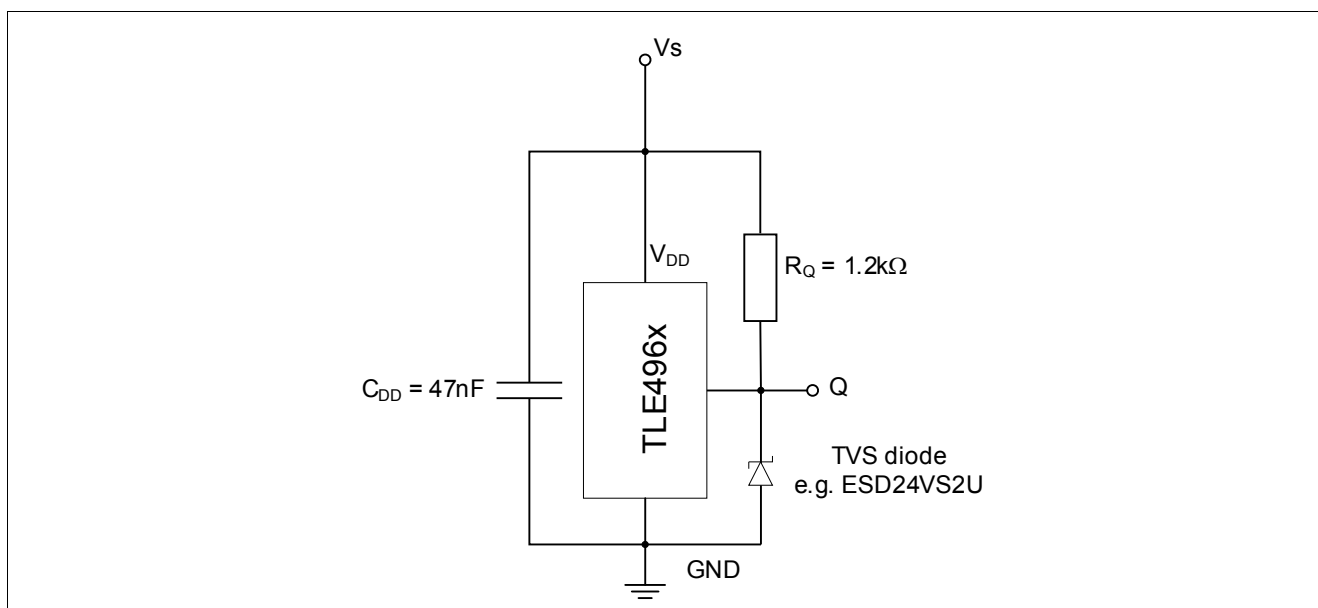
Figure 3-2 Application Circuit #2 for extended ESD robustness
