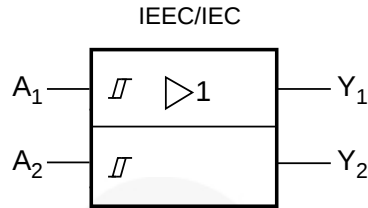
Figure 1. Logic Symbol
