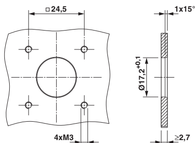
Installation dimensions
