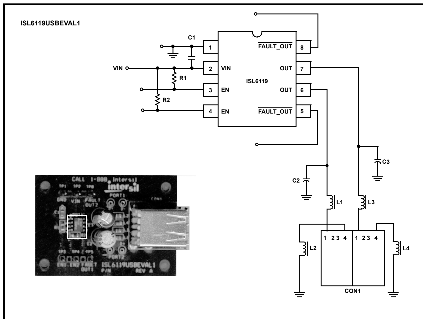
FIGURE 20. ISL6119USBEVAL BOARD
