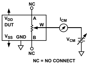
Figure 33. Common-Mode Leakage Current
