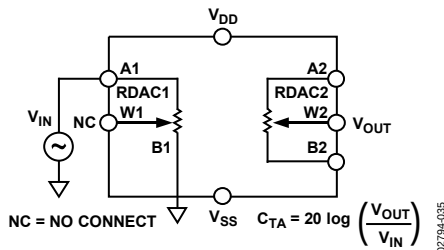
Figure 34. Analog Crosstalk
