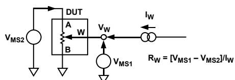
Figure 27. Wiper Resistance
