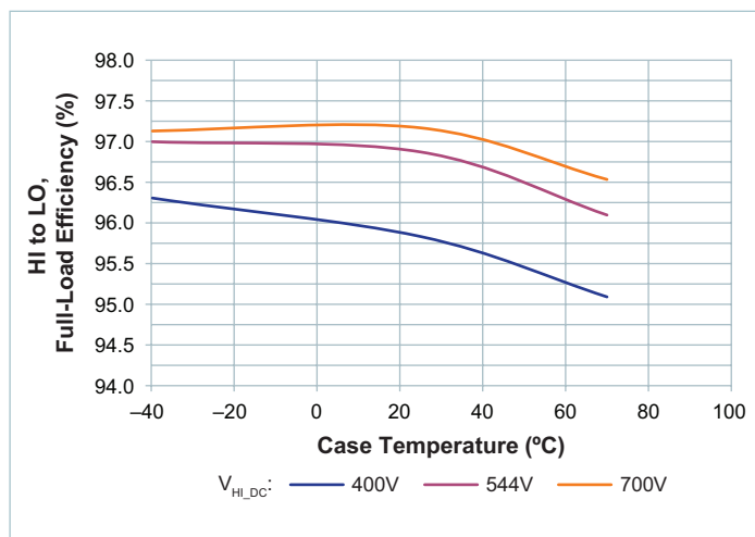
Figure 5 — Full-load efficiency vs. temperature
