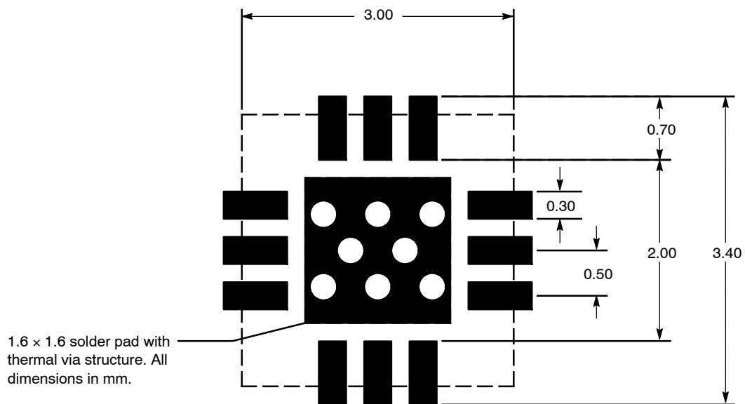
Figure 45. PCB Pad Layout for QFN 3 × 3
