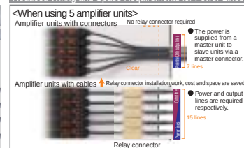
Reduced Wiring and Space Requirements for Power Lines
