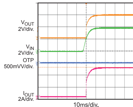
V_{IN} Startup
