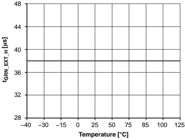
Figure 15. tGRN_EXT_H
