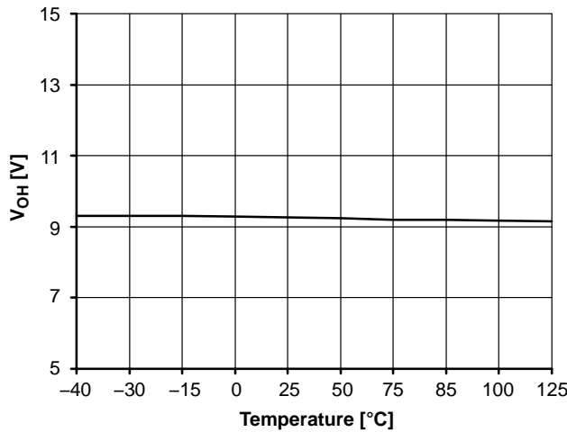
Figure 19. VOH
