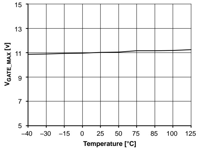
Figure 18. VGATE_MAX
