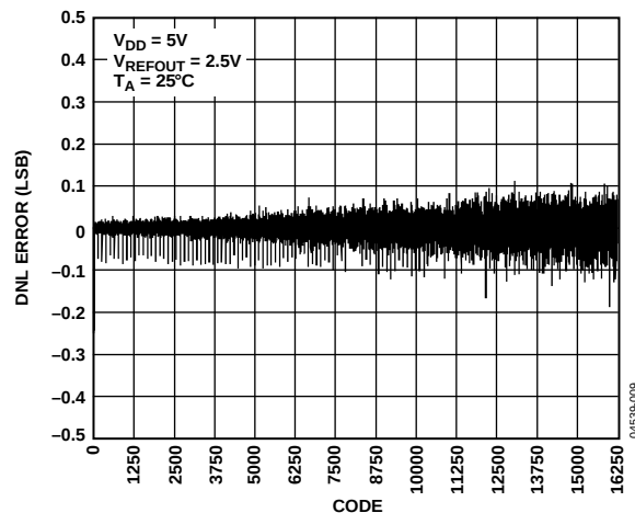
Figure 9. DNL—AD5640-2/AD5640-3
