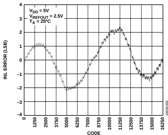
Figure 6. INL—AD5640-2/AD5640-3
