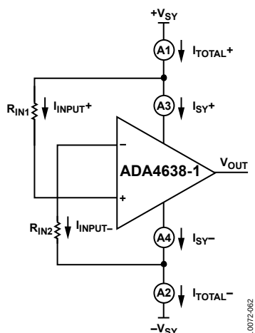
Figure 62. Comparator B
