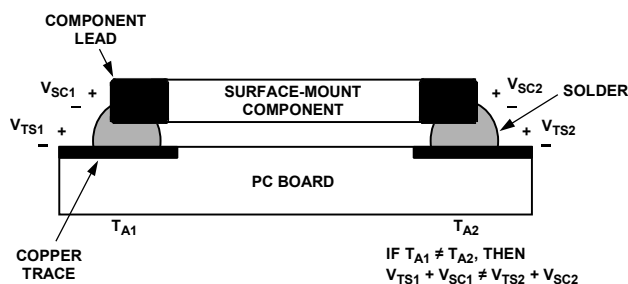
Figure 68. Mismatch in Seebeck Voltages Causes Seebeck Voltage Error
