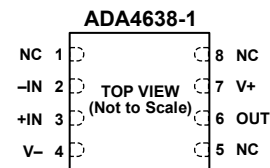
Figure 1. 8-Lead SOIC
