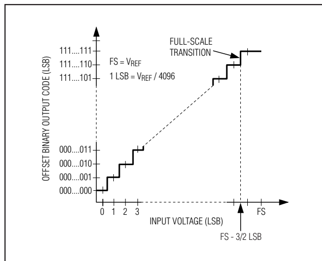
Figure 3. Unipolar Transfer Function—Full Scale (FS) = V_{REF}
