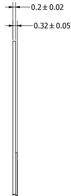
A (9 : 1)
