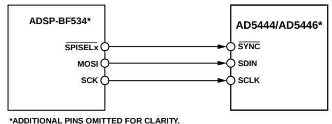
Figure 47. ADSP-BF534 to AD5444/AD5446 Interface
