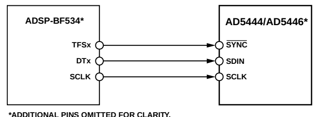
Figure 48. ADSP-BF534 to AD5444/AD5446 Interface
