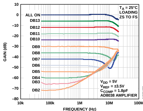
Figure 22. Reference Multiplying Bandwidth vs. Frequency and Code
