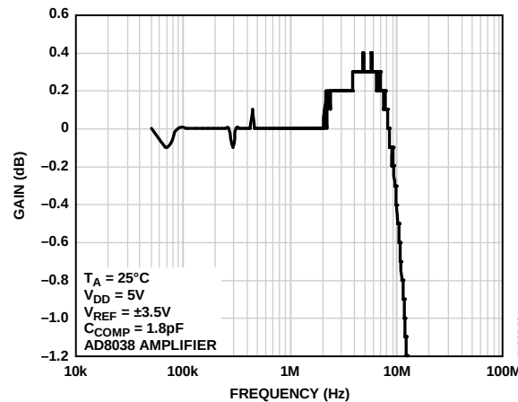
Figure 23. Reference Multiplying Bandwidth vs. Frequency—All 1s Loaded
