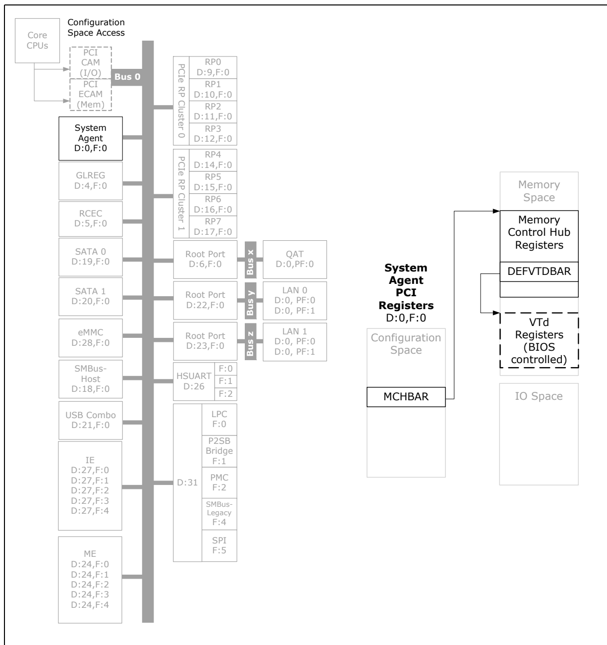
Figure 5-2. Register Map
