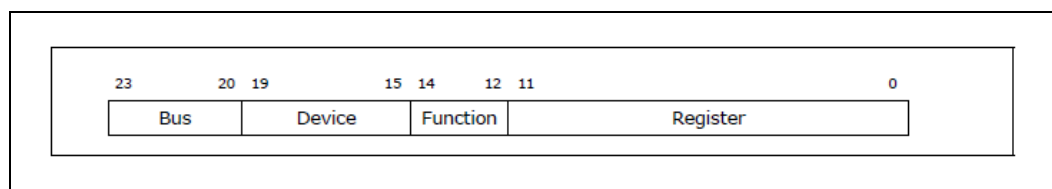
Figure 30-8. PCI Configuration Address Format
