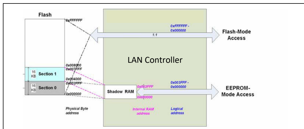
Figure 13-4. Shared SPI Flash Shadow RAM
