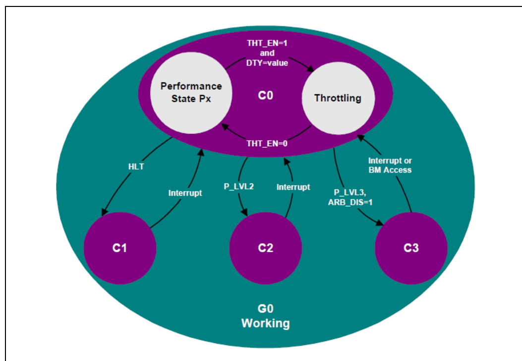
Figure 34-3. Processor Power States
