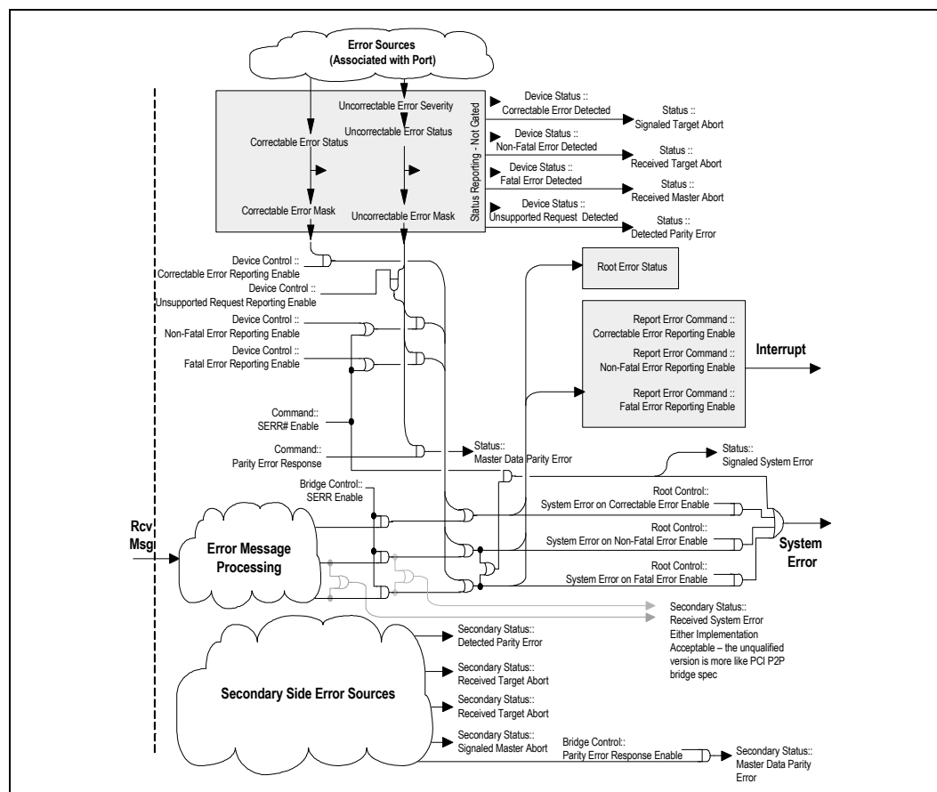
Figure 13-3. Error Reporting Mechanism
