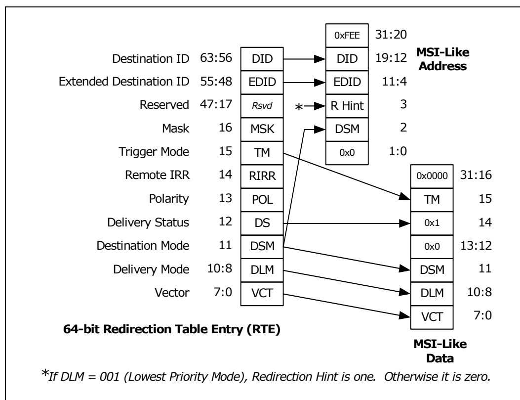
Figure 21-3. MSI-Like IOxAPIC Interrupt Message for the Local APICs
