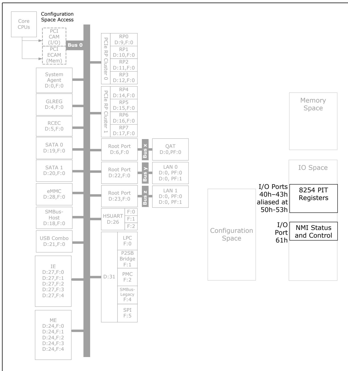
Figure 23-3. Register Map
