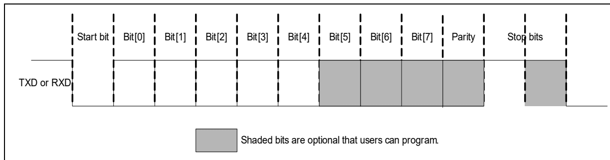
Figure 18-4. UART Data Transfer Flow
