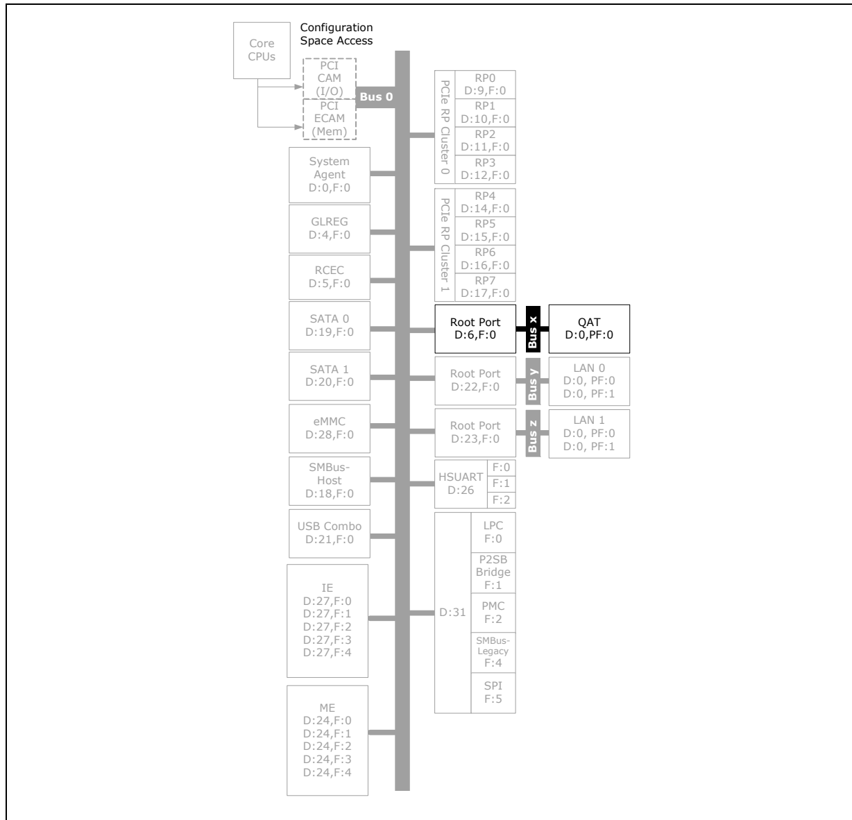
Figure 31-5. Register Map
