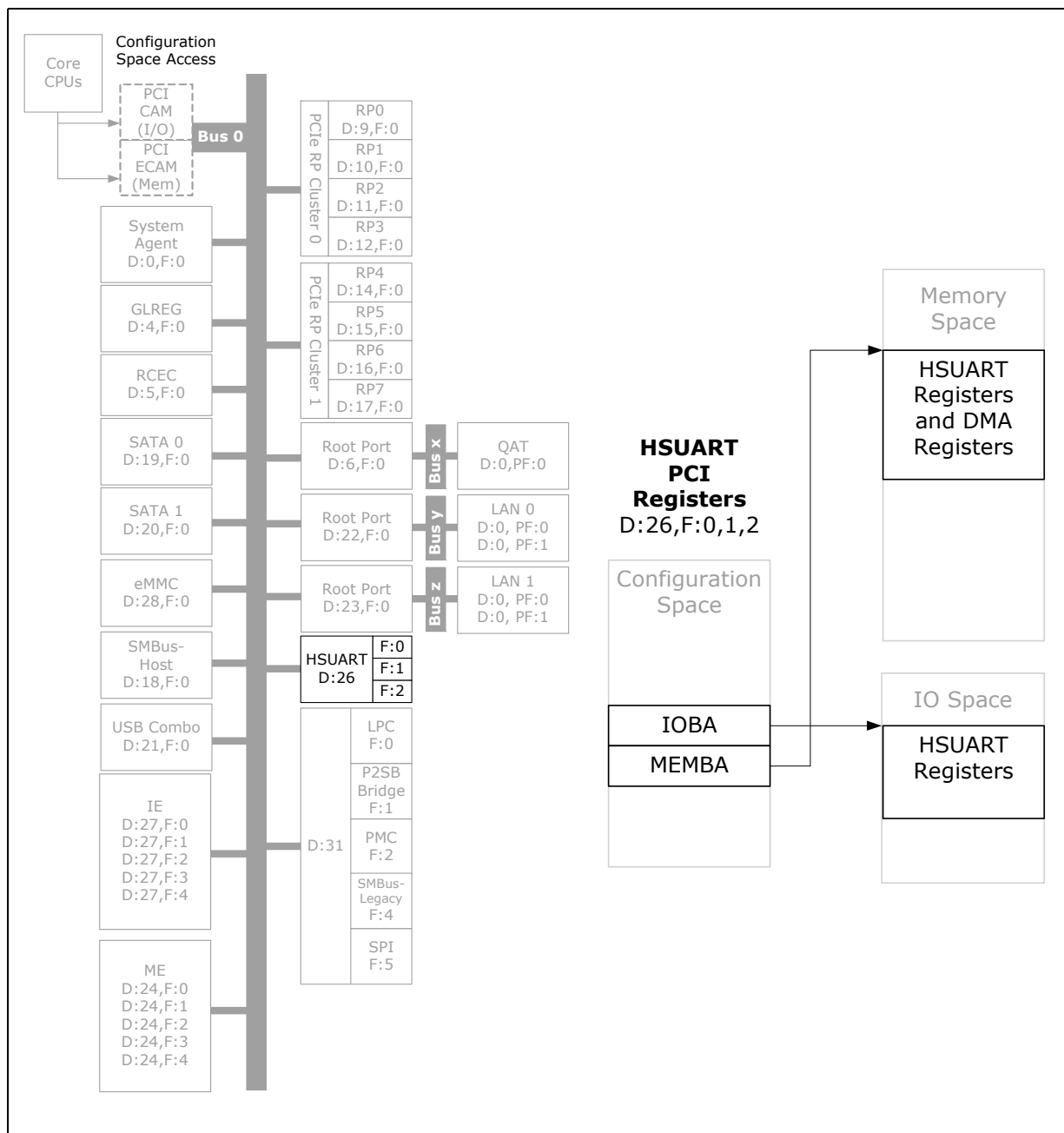
Figure 18-9. Register Map
