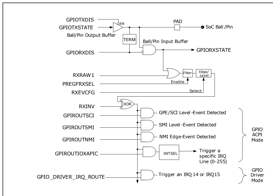
Figure 26-3. GPIO Logic Overview Diagram
