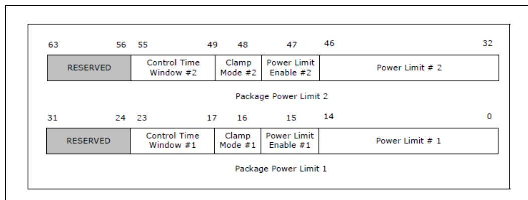
Figure 30-29. Package Turbo Power Limit Data
