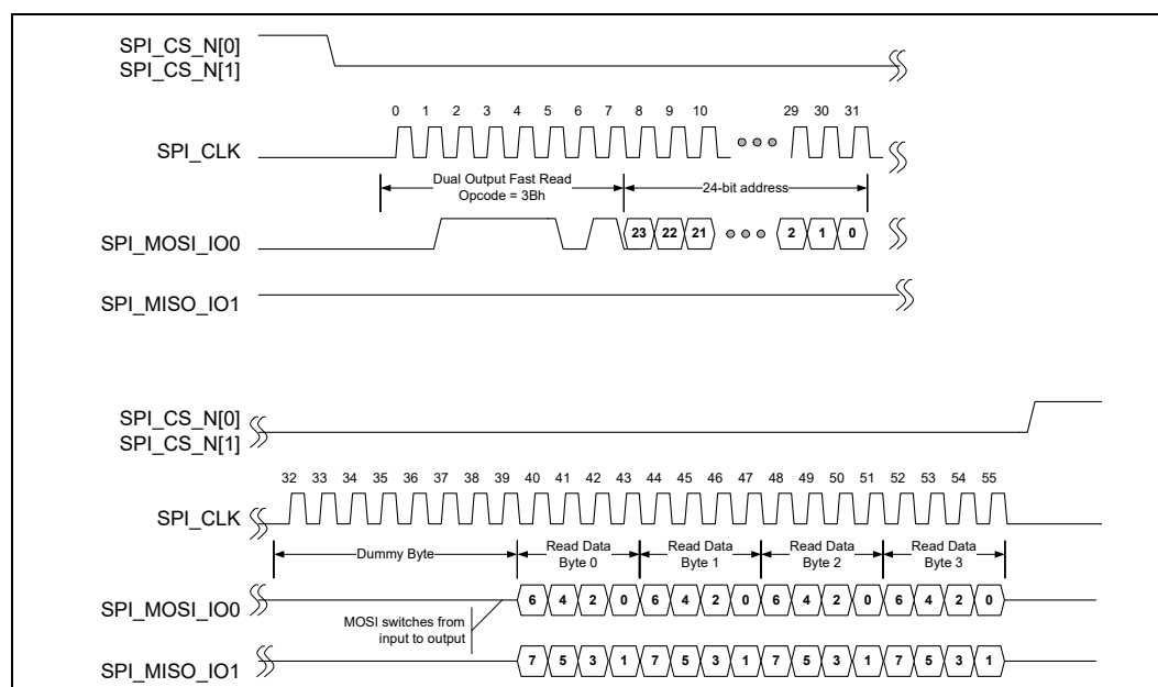
Figure 19-6. Dual-Output-Fast-Read Timing
