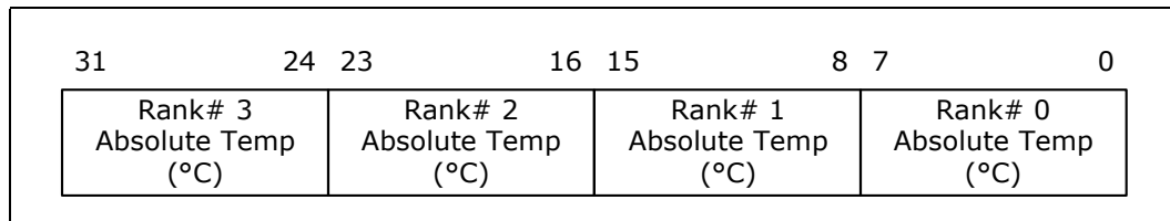
Figure 30-10. Write DRAM Rank Temperature Data Dword
