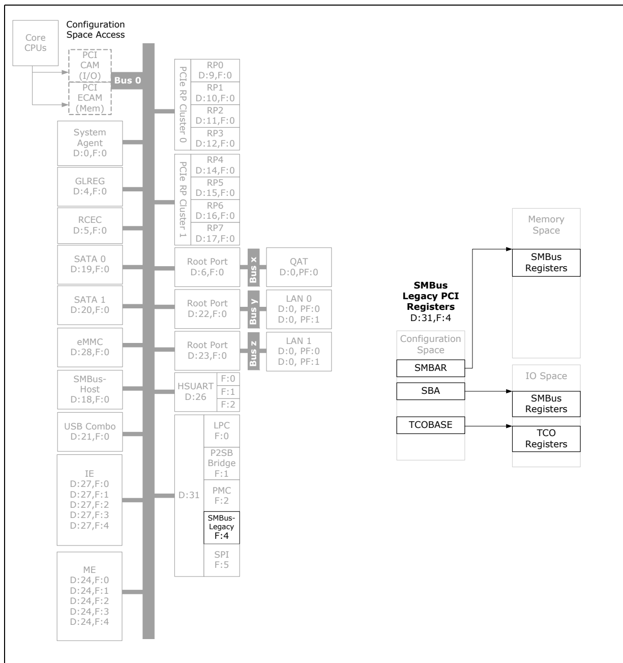
Figure 28-2. Register Map
