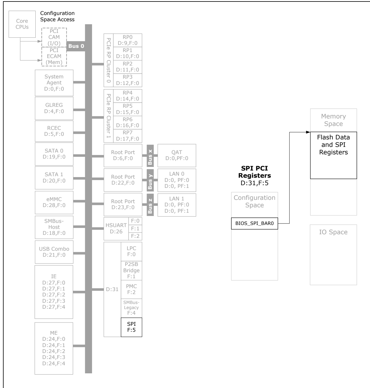
Figure 19-10. Register Map
