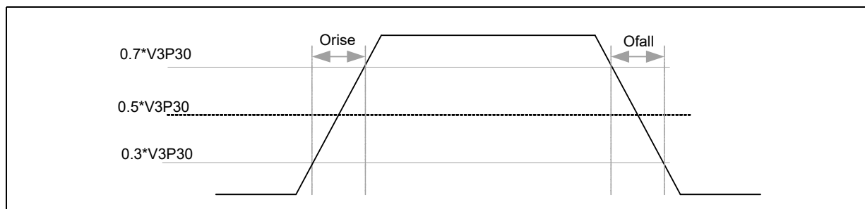
Figure 40-9. 3.3V GPIO Driver Timing
