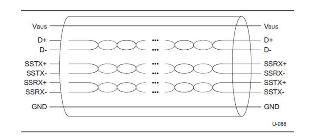
Figure 14-2. USB 3.0 Cable
