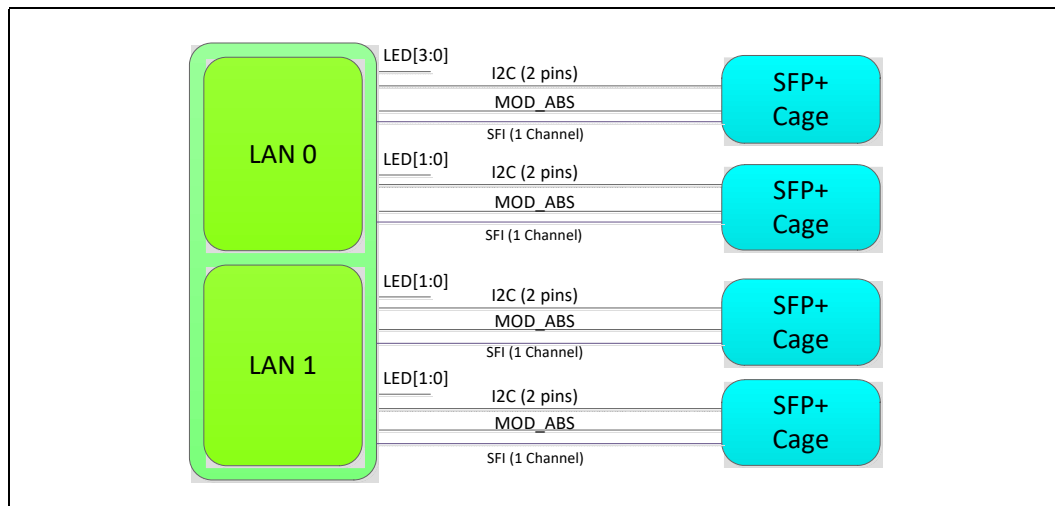
Figure 13-7. SFP+ Implementation
