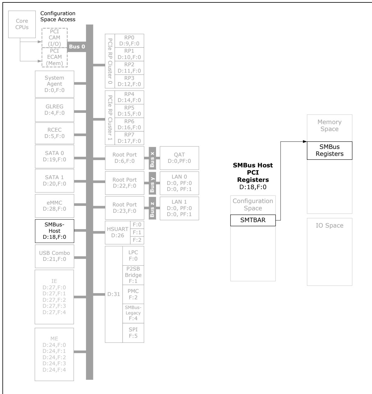
Figure 29-16. Register Map
