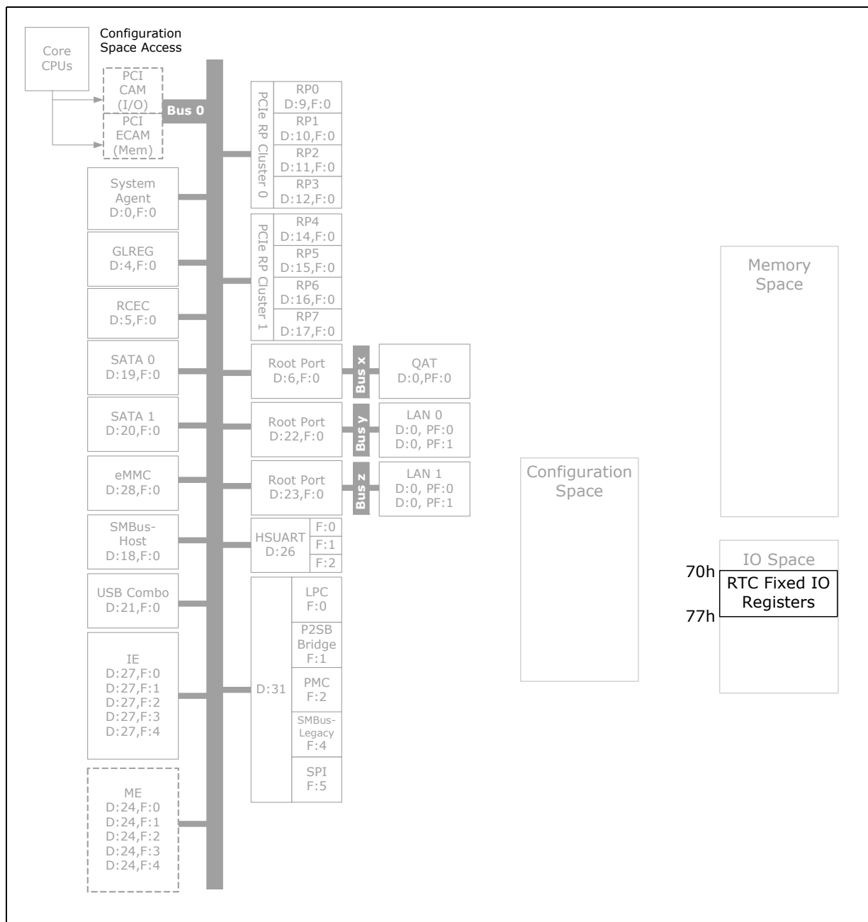
Figure 24-2. Register Map
