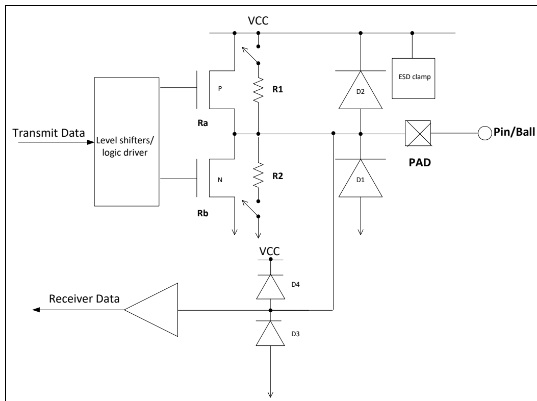
Figure 26-2. Custom GPIO Circuit Definition
