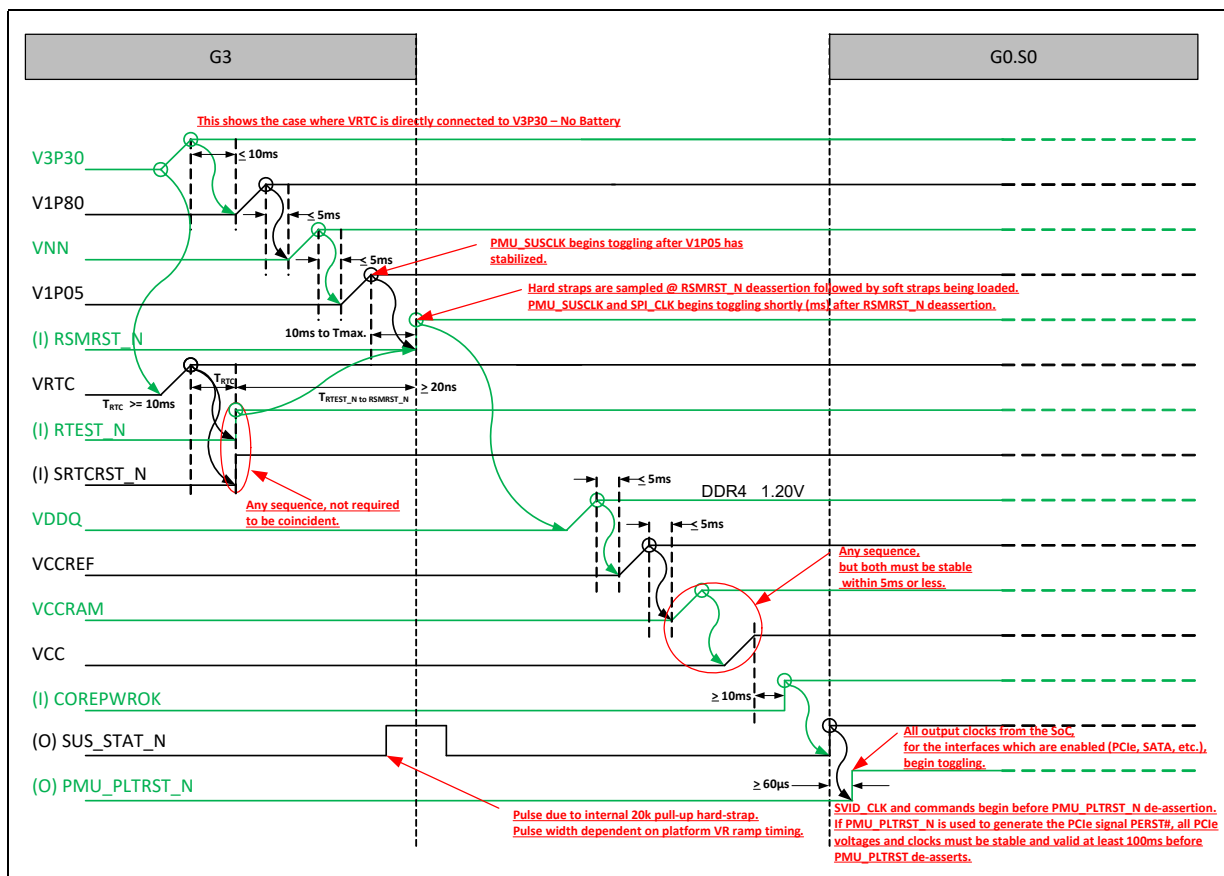
Figure 33-2. Non-ACPI Cold Boot Sequence
