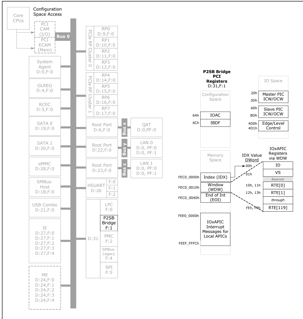
Figure 21-4. Register Map
