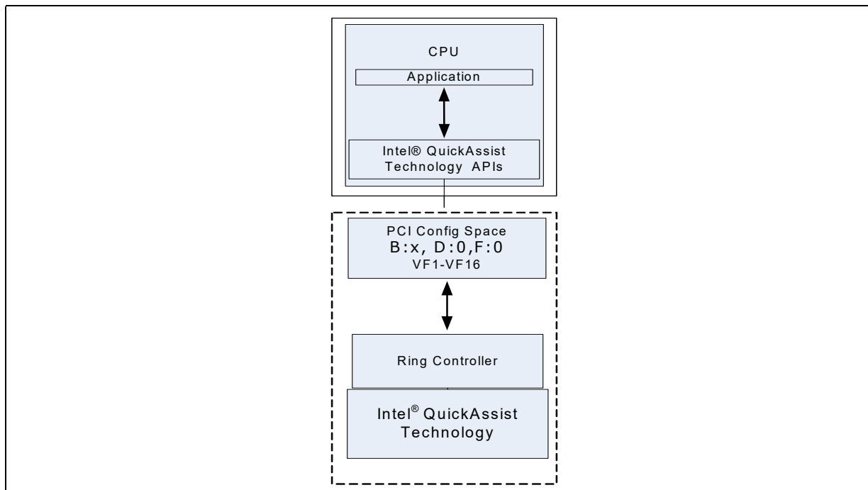
Figure 31-2. Intel® QAT Usage Block Diagram
