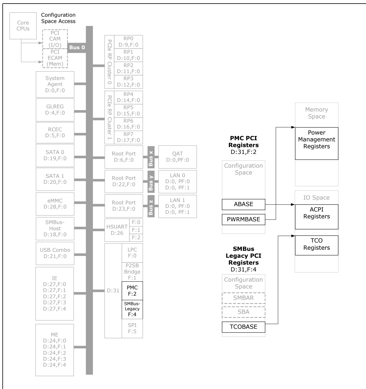
Figure 16-2. Register Map
