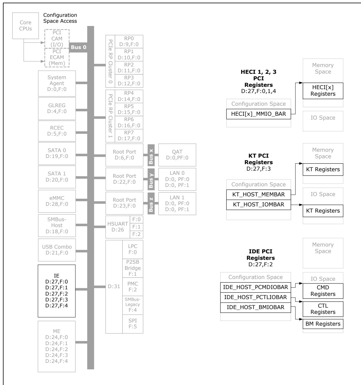
Figure 37-4. Register Map
