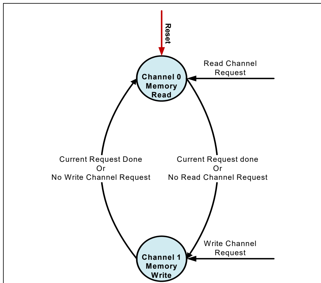
Figure 18-7. Logical Representation of Channel Arbitration
