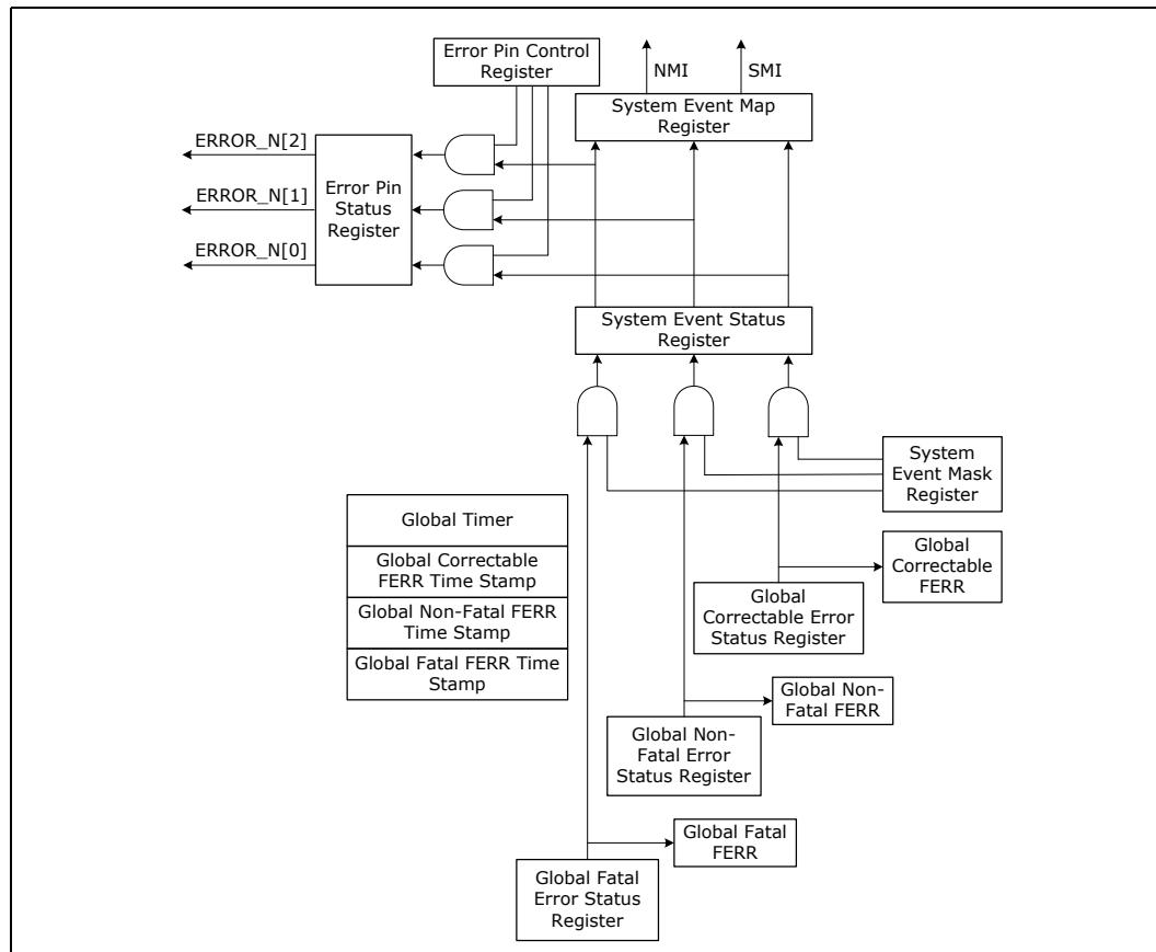
Figure 6-7. Global Error Registers and System Event Reporting
