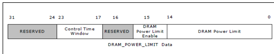
Figure 30-15.DRAM Power Limit Data
