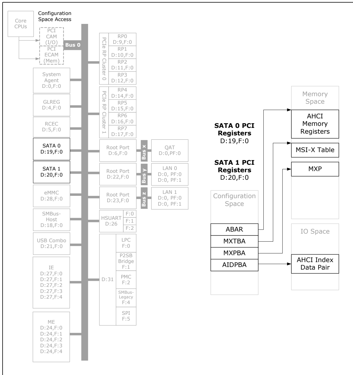
Figure 12-2. Register Map
