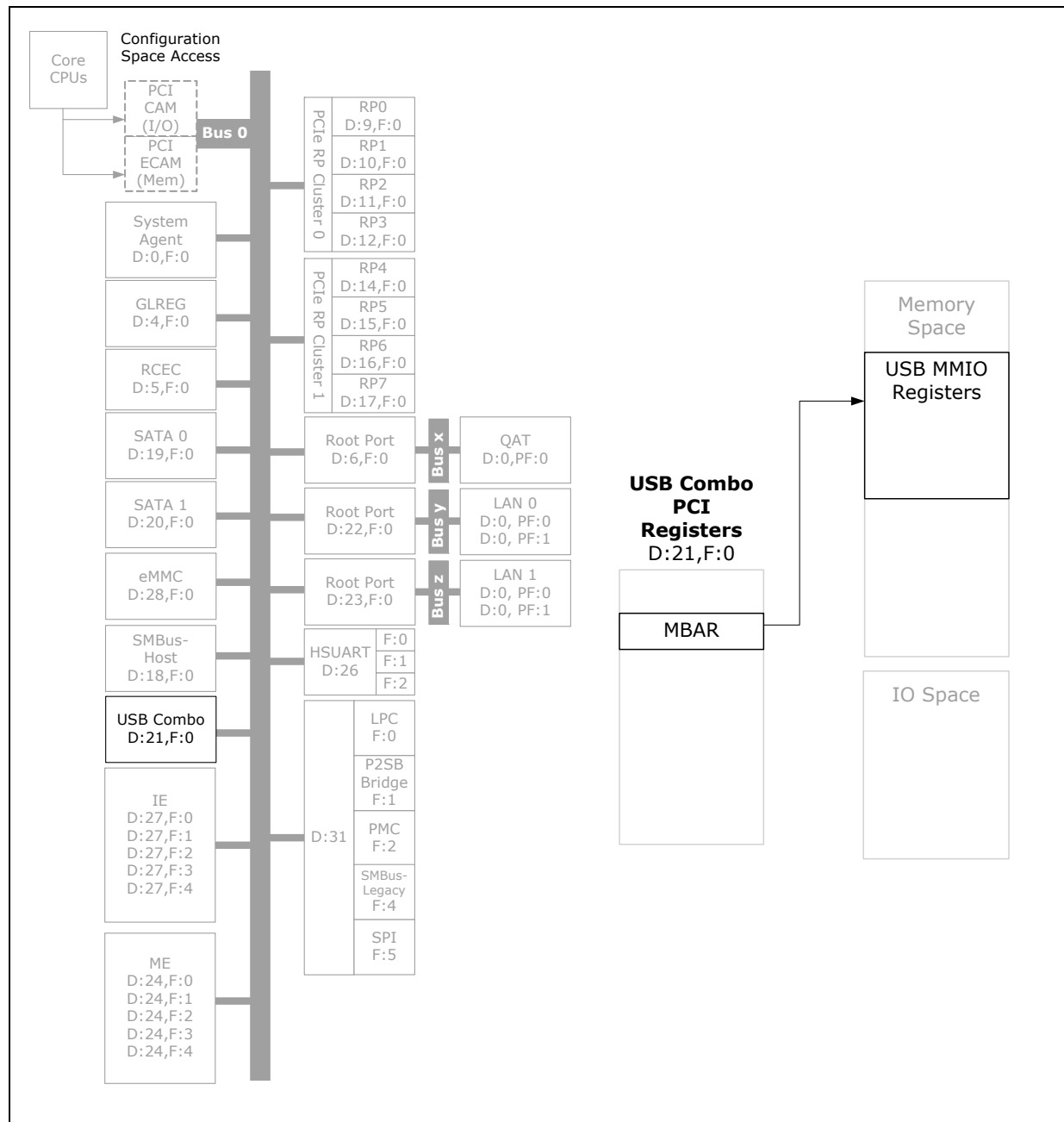
Figure 14-6. Register Map
