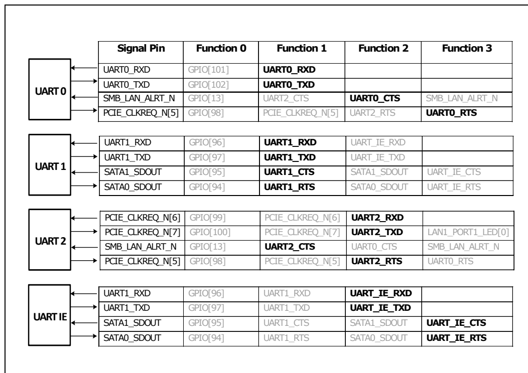
Figure 18-2. UART MUXed Signals
