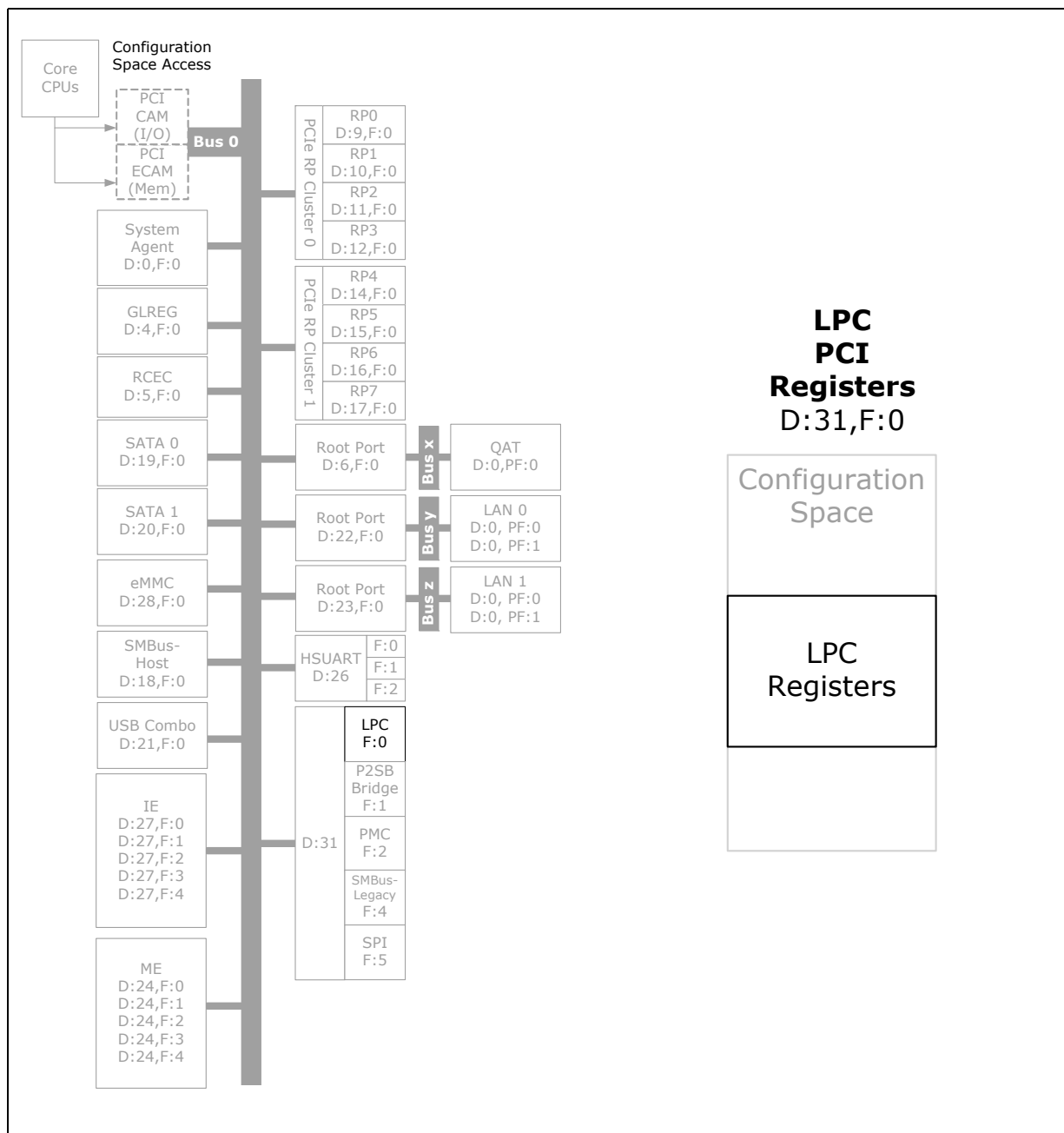
Figure 20-3. Register Map
