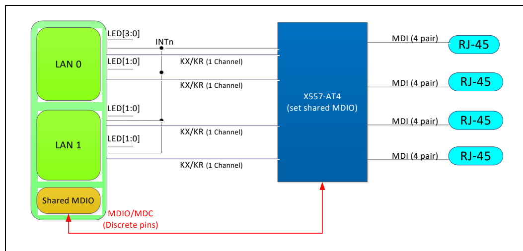
Figure 13-5. 10GBASE-T Implementation
