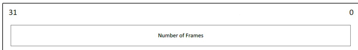
Figure 30-40. Crash Dump Capabilities (Parameter0 = 0x1)
