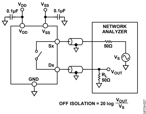
Figure 34. Off Isolation
