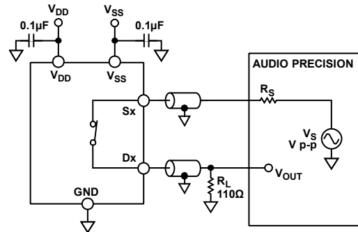
Figure 38. THD + N
