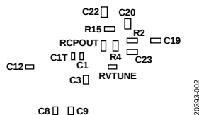
Figure 2. Loop Filter Component Placement
