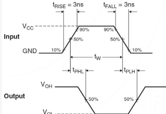
Figure 5. AC Waveforms
