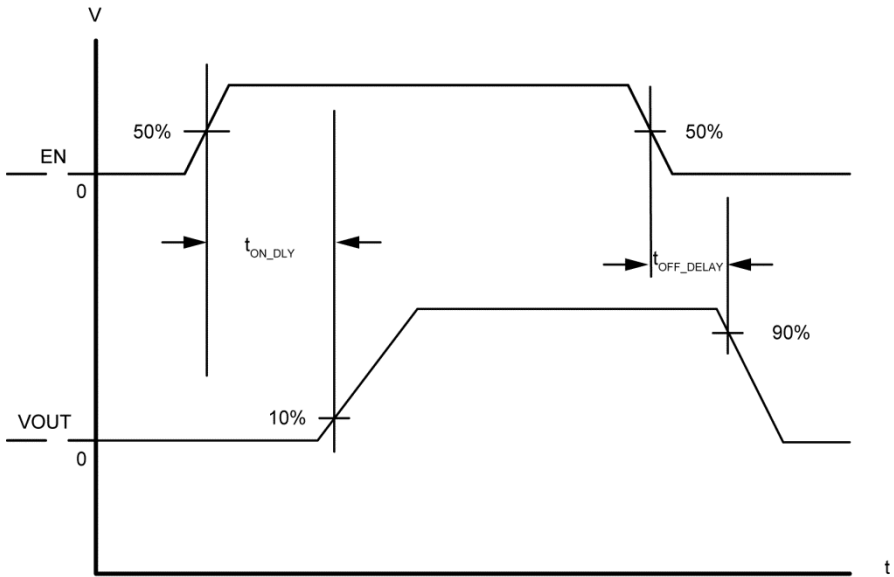
Figure 2. Turn-On/Off Delay
