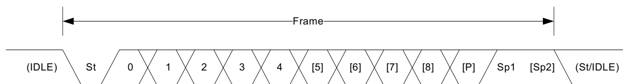
Figure 25-2. Frame Formats
