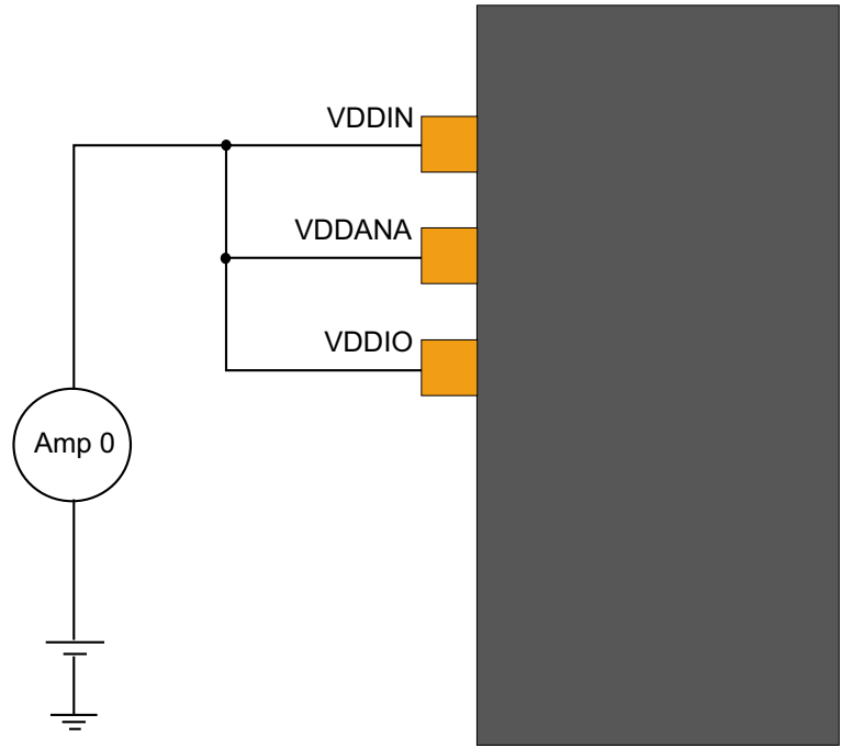
Figure 39-1. Measurement Schematic
