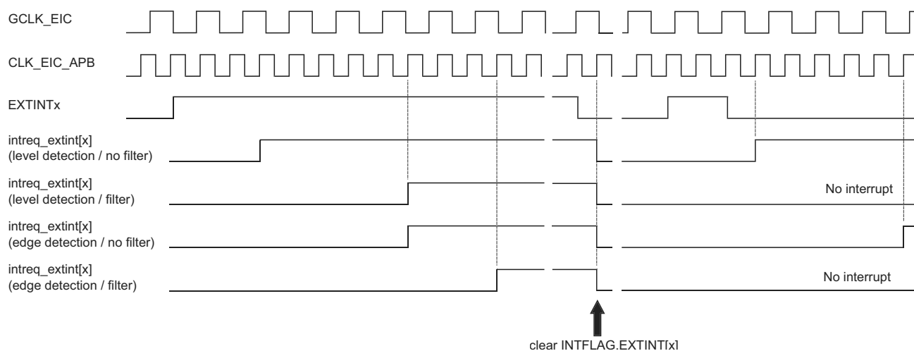
Figure 20-2. Interrupt detections
