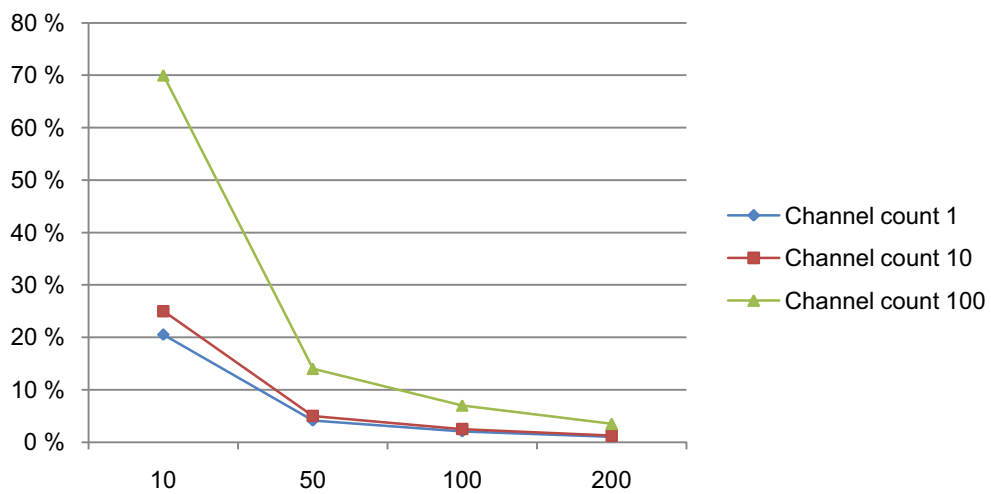
Figure 34-13.CPU utilization.
