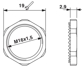
Dimensioned drawing
