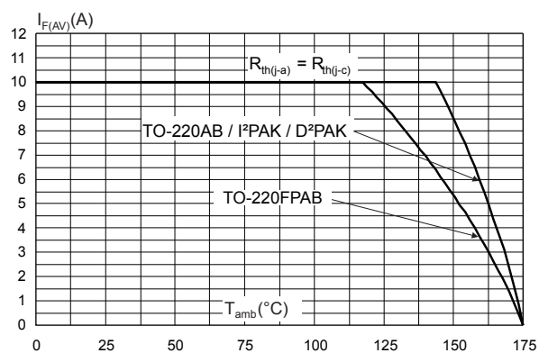
Figure 12. Average forward current versus ambient temperature ( \delta = 0.5 , per diode)
