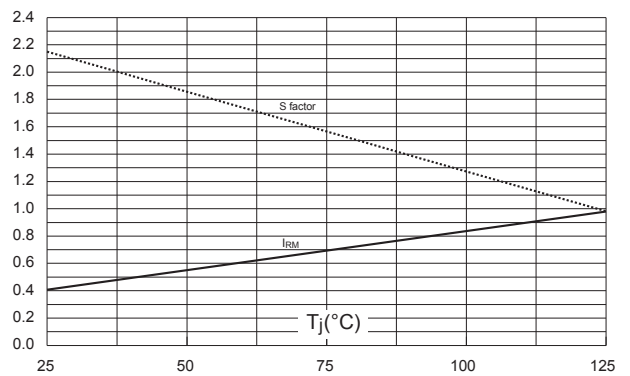
Figure 8. Relative variation of dynamic parameters versus junction temperature (reference: T_J = 125^\circ\text{C} )
