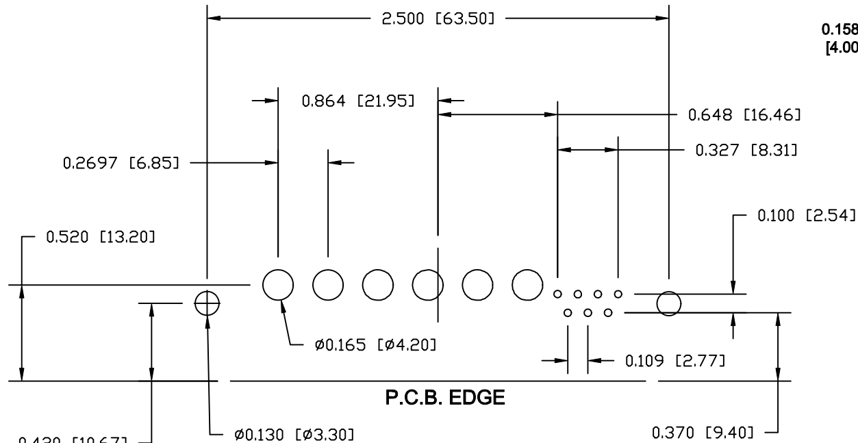
PCB LAYOUT
