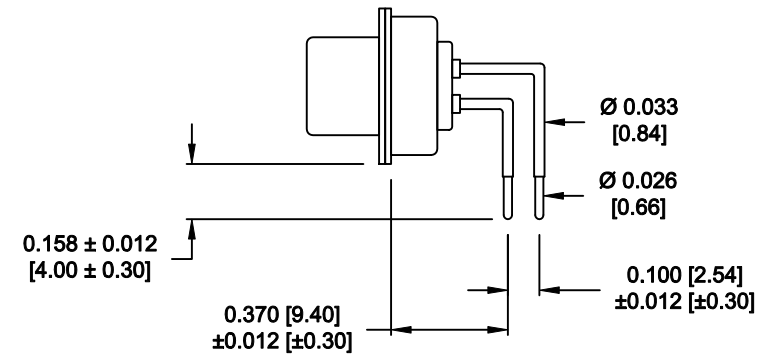
SIGNAL CONTACTS
