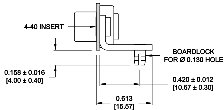
MOUNTING HARDWARE
