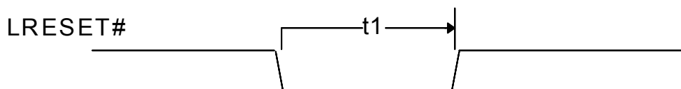
FIGURE 38-7: RESET TIMING
