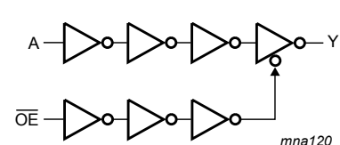
Figure 3. Logic diagram
