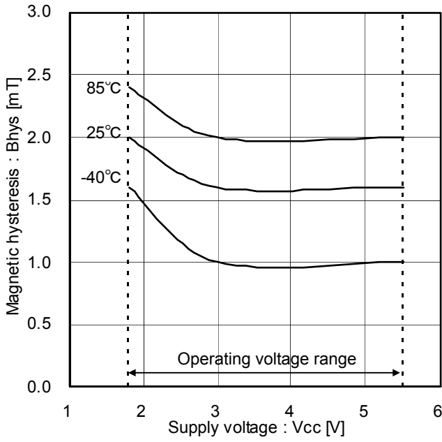
Figure 7. Magnetic hysteresis
