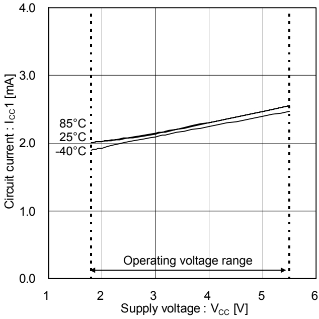
Figure 3. Circuit Current 1
