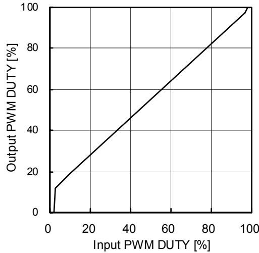
Figure 21. Characteristic of input PWM DUTY and output PWM DUTY
