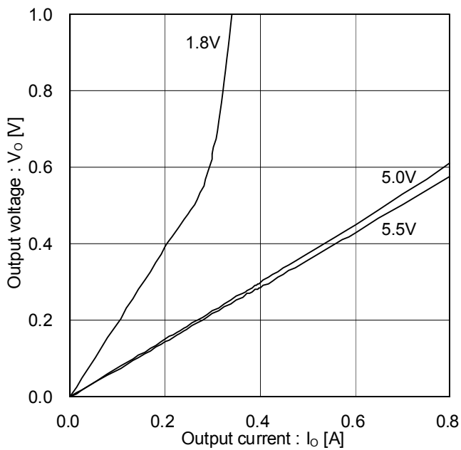
Figure 13. Total Output Voltage (Output H and L) (Voltage Characteristics)
