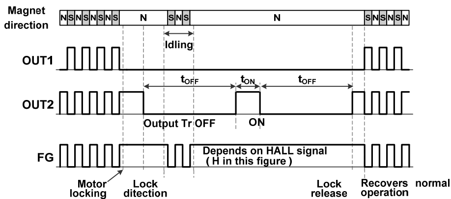
Figure 26. Lock protection timing chart
