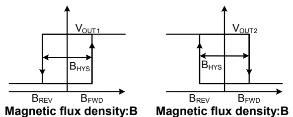
Figure 2. Output operation
