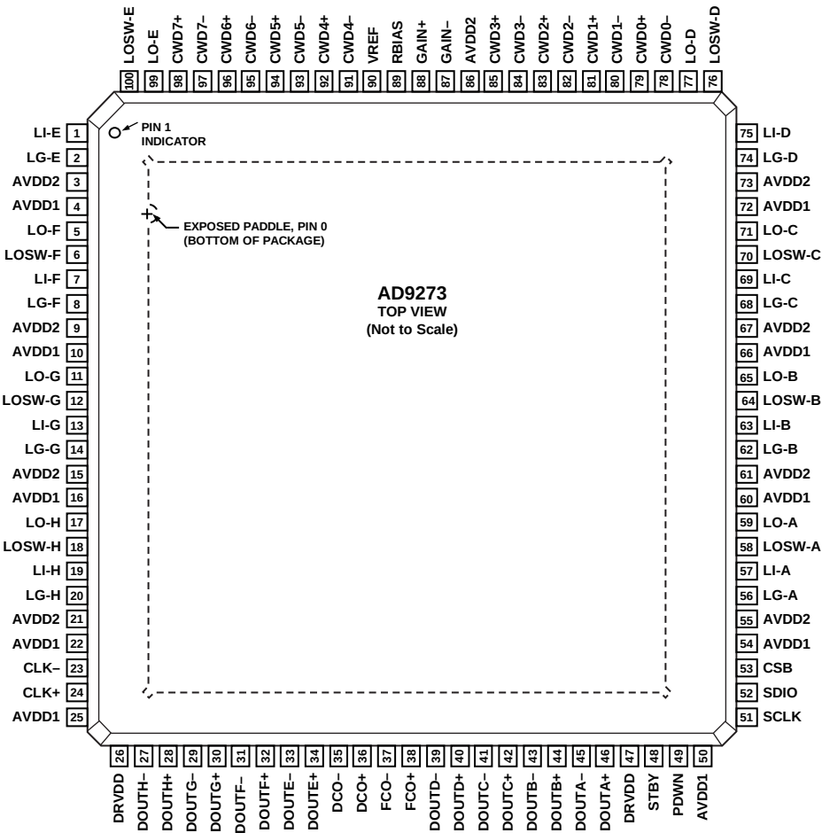
Figure 4. TQFP Pin Configuration
