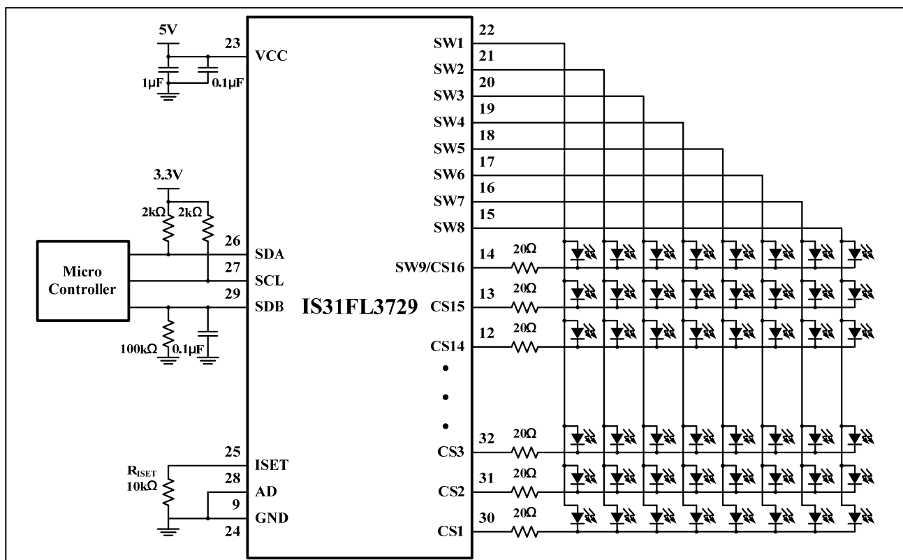
Figure 1 Typical Application Circuit (16×8)
