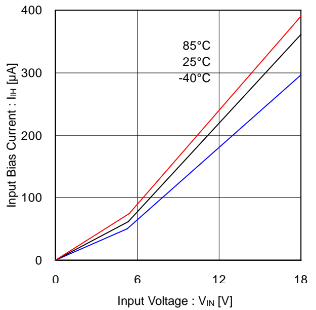
Figure 12. Input Bias Current vs Input Voltage
