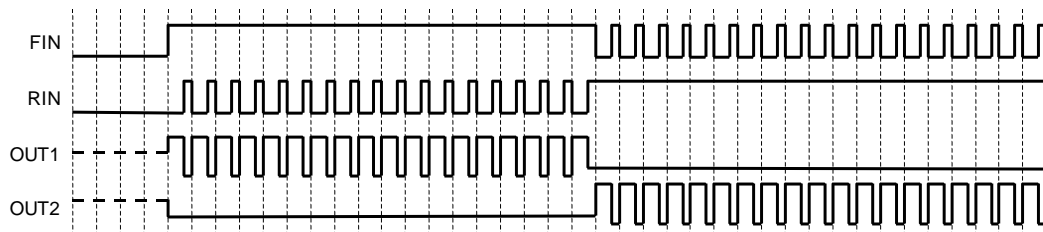
Figure 37. PWM Control Mode B Operation (Timing Chart)
