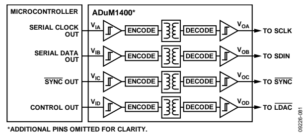
Figure 88. Isolated Interface
