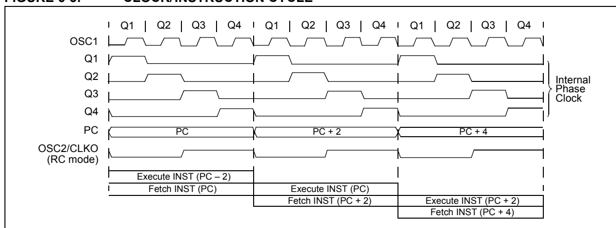
FIGURE 6-3: CLOCK/INSTRUCTION CYCLE
