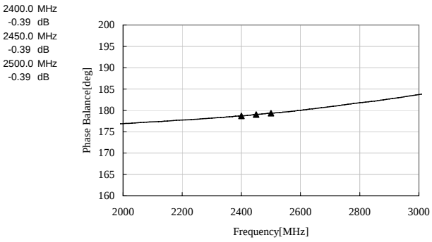
Phase Balance
