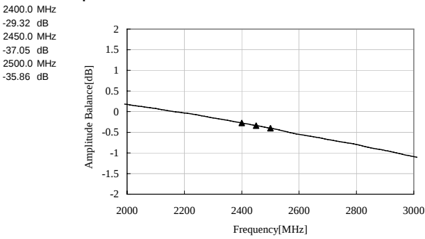
Amplitude Balance
