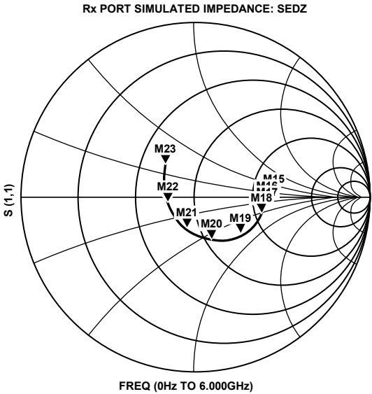
Figure 429. Receiver Input Impedance SEDZ
