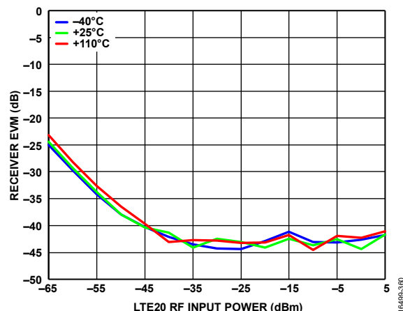
Figure 235. Receiver EVM vs. LTE20 RF Input Power, LTE = 20 MHz RF Signal, LO = 600 MHz
