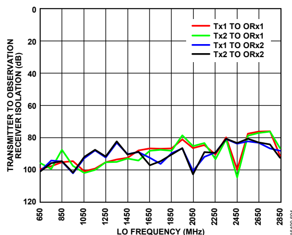
Figure 192. Transmitter to Observation Receiver Isolation vs. LO Frequency, Temperature = 25°C
