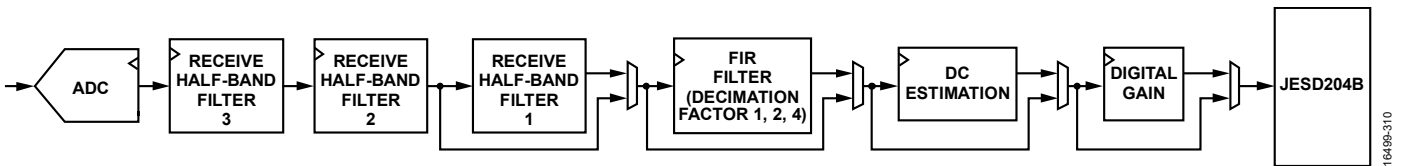
Figure 431. Receiver and Observation Receiver Datapath Filter Implementation
