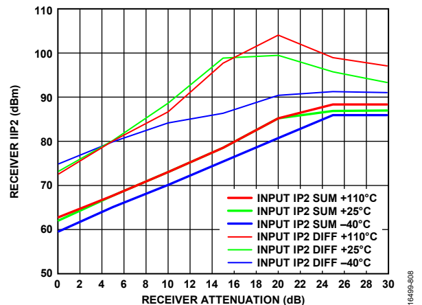
Figure 305. Receiver IIP2 vs. Receiver Attenuation, LO = 4600 MHz, Tones Placed at 4645 MHz and 4646 MHz, -21 dBm Plus Attenuation
