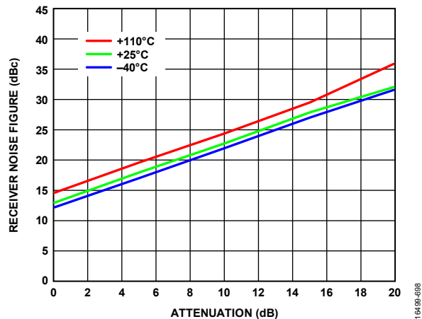
Figure 196. Receiver Noise Figure vs. Attenuation, LO = 1850 MHz, Receiver Bandwidth = 200 MHz Bandwidth, Sample Rate = 245.76 MSPS, Integration Bandwidth = 500 kHz to 100 MHz
